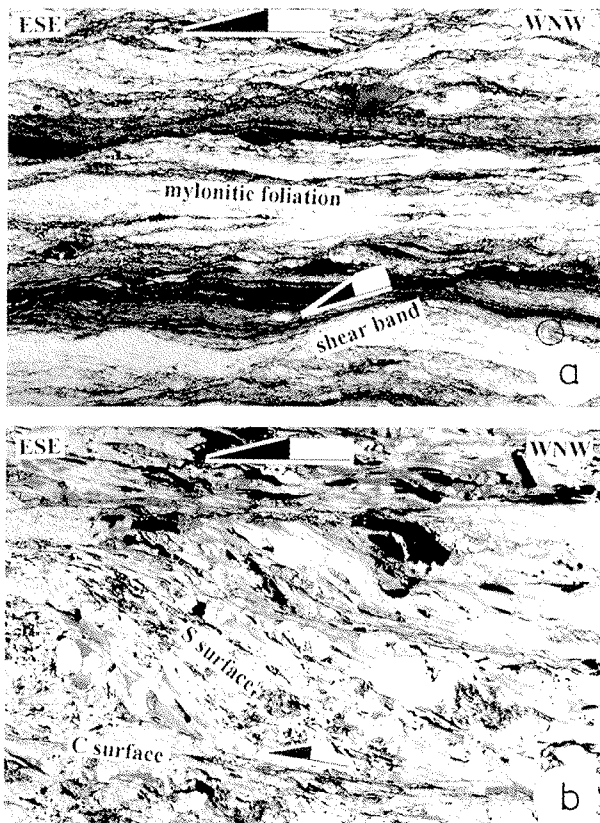
Fig. 7 Examples of microstructures indicating top-to-the-ESE displacement within the Murau nappe. (a) Mylonitic quartzphyllite with shear bands. (b) S-C fabrics. Long edge of both photomicrographs: ca. 4 mm. Crossed polarizers.
