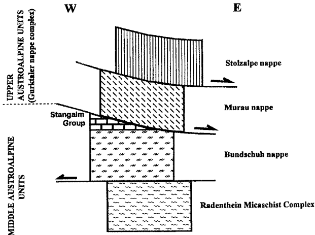
Fig. 3 Schematic tectonic stratigraphy of the investigated area.
