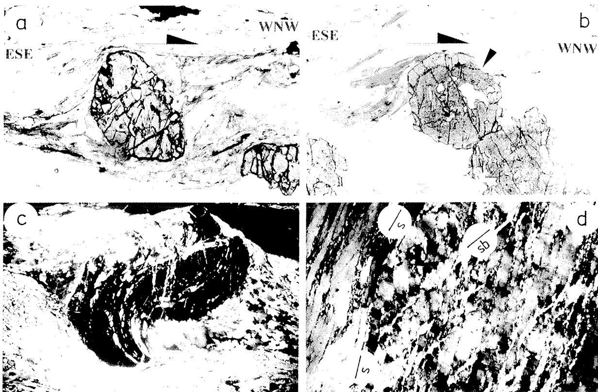
Fig. 5 Comparison of microfabies in the Middle and Upper Austroalpine units: (a) Mantled garnet from the Radenthein micaschist with asymmetric quartz tails indicating top-to-the-WNW shear (BK1). (b) Zoned garnet from a gneiss of the Bundschuh nappe (BK10). (c) Garnet-bearing quartz-phyllite with \sigma -type garnet porphyroclast indicating top-to-the-E transport. Note the wrapping of foliation around the garnet (Gurktaler phyllite of the Murau nappe, sample BK7). (d) quartz microfabric of the Murau nappe (sample BK3). Note large elongated quartz grains and formation of shear bands with recrystallized small quartz grains. Long edge of all four photomicrographs: ca. 4 mm. Crossed polarizers.
